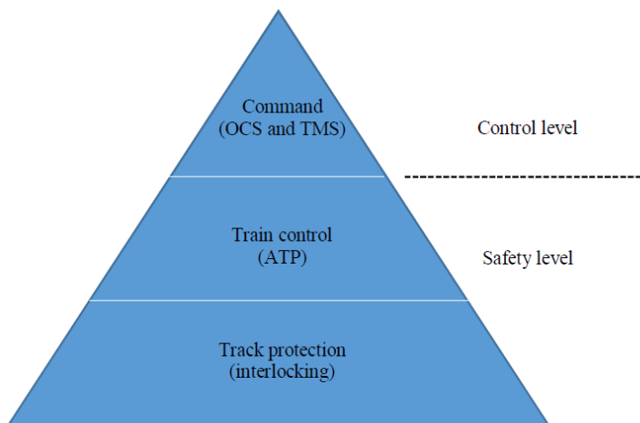
Figure 11: Elements of mainline signalling systems
