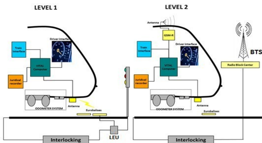
Figure 12: Overview of ETCS (Level 1 and Level 2)
